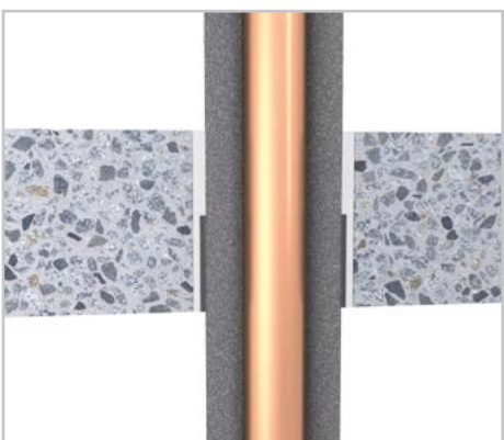
Non-combustible pipes with wrap into the floor
